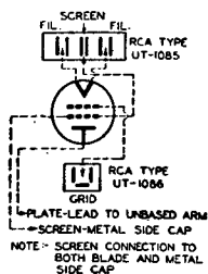
Connections to End-Mountings
