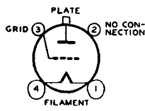
Top View of Socket Connections
