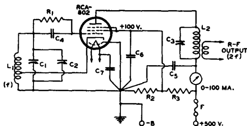
ELECTRON-COUPLED OSCILLATOR
