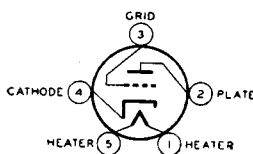
RCA-843
