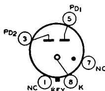
G-4R Type 0Z4-G
