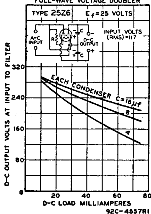
OPERATION CHARACTERISTICS FULL-WAVE VOLTAGE DOUBLER
