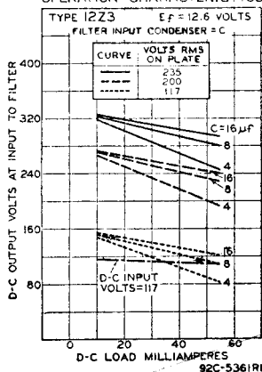
OPERATION CHARACTERISTICS
