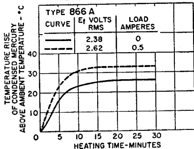
RATE OF RISE OF CONDENSED-MERCURY TEMPERATURE
