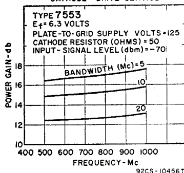
GAIN CHARACTERISTICS CATHODE-DRIVE SERVICE
