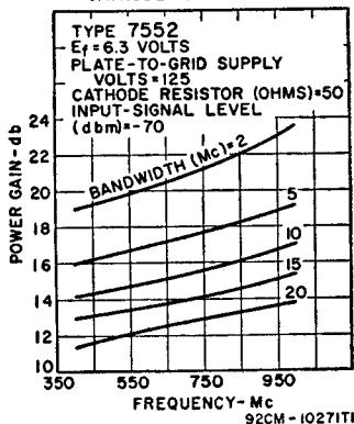
GAIN CHARACTERISTICS CATHODE-DRIVE SERVICE
