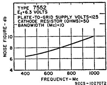
NOISE FIGURE CHARACTERISTIC CATHODE-DRIVE-SERVICE
