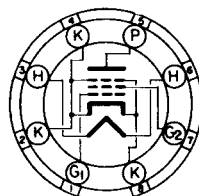
BOTTOM VIEW SUBMINIATURE BUTTON 8 FLEXIBLE LEADS 80L
