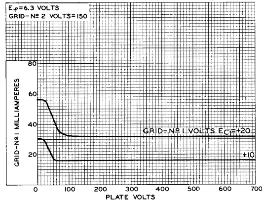
Fig. 5 - Typical Characteristics of Type 6146A.
