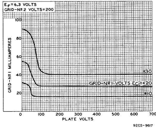
Fig.2 - Typical Characteristics of Type 6146A.
