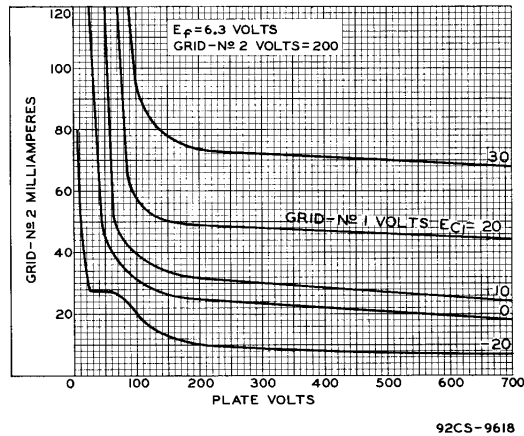
Fig.3 - Typical Characteristics of Type 6146A.
