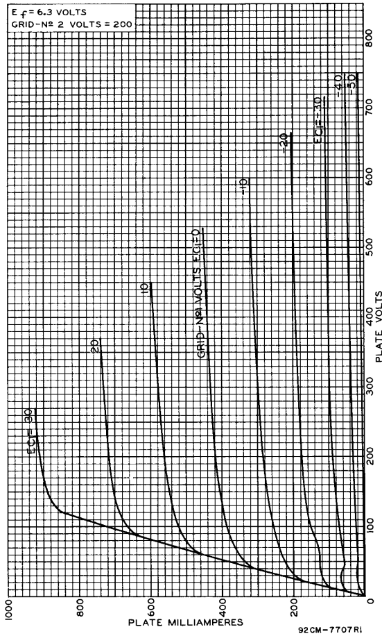
Fig.1 - Typical Plate Characteristics of Type 6146A.
