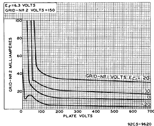
Fig. 6 - Typical Characteristics of Type 6146A.
